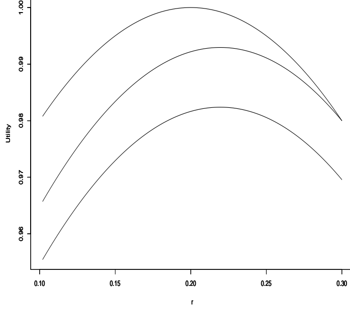
FIGURE 1. The top curve is the utility as a function of r and W_t = 1 . This has optimum for \tilde{r} = 0.2 . The two other curves show the utility that may be obtained from a rebalance from r_{t-} = 0.3 . The top one of these has only proportional transaction fee while the lowest also has flat fee. Notice that both of these curves have optimum for the same value r that is the upper bound of the no-trade region with only proportional costs. The maximum of the lowest curves is equal to U(0.3) , illustrating that the boundary of the no-trade region including both proportional and flat transaction costs is 0.3. Since the two curves at the bottom are quite flat close to the optima, we see that the exact position of the no-trade region is not critical.
